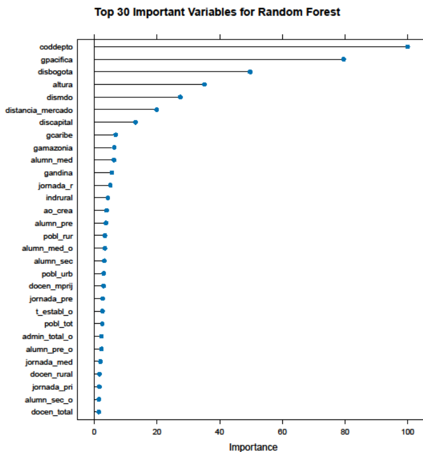
Figure 2. Important features of the estimation
