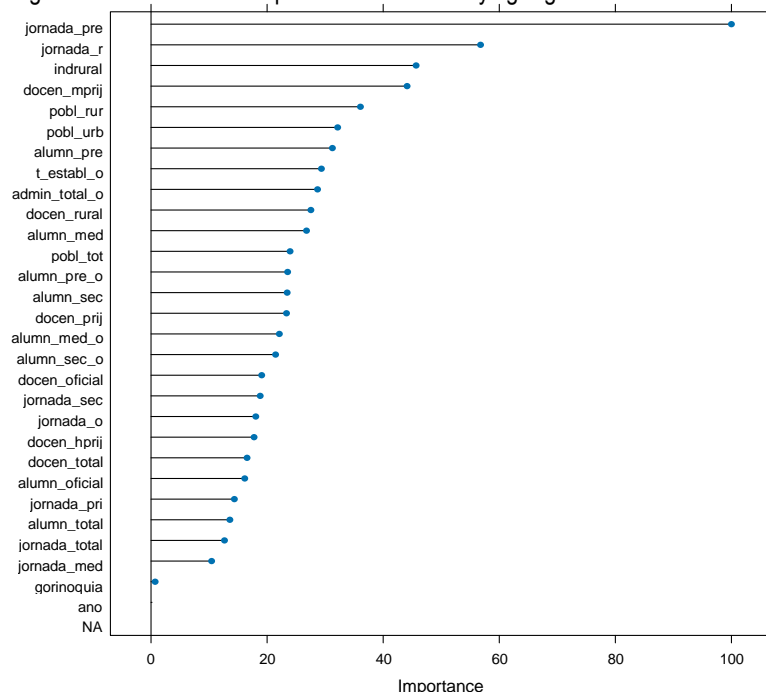
Figure 7. Model estimation performance with varying regressors
