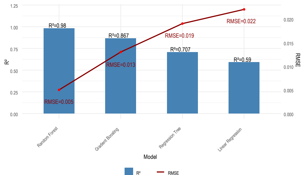
Figure 1. Model estimation performance
