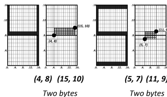
Figure 1. Digits "4" and "5" and their sub-interval images namely their standard cuboids ( CboGs ) of gravity
