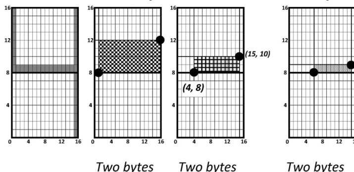
Figure 6. The CboG concentric S-IIs of the digit "4". The concentric central S-I weights equal 1/2, 1/4, 1/8
