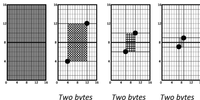
Figure 5. The concentric CboG S-IIs of the uniform picture. The central concentric S-I weights equal 1/2, 1/4, 1/8
