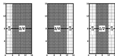
Figure 4. The formation of three horizontal sub-intervals for the standard CboG 1/4 : 1/2 : 1/4 on the uniform picture
